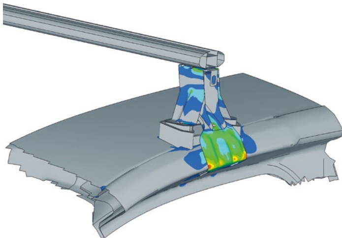
Simulation map of stress induced by roof rack tightening.
